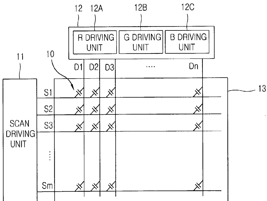
FIG. 2 CONVENTIONAL ART
